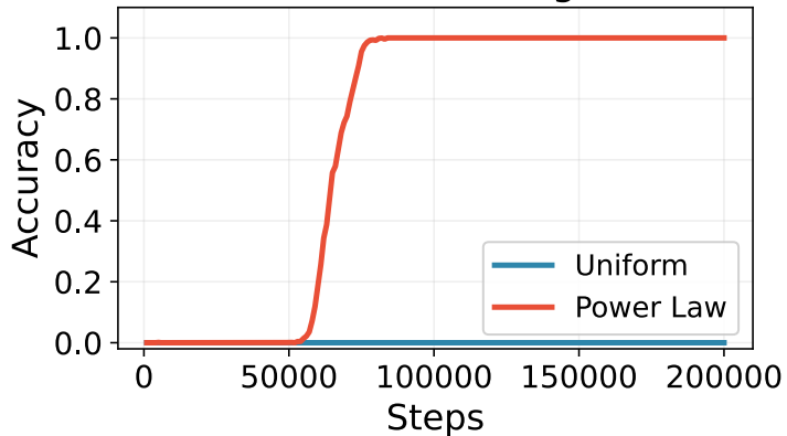
State Tracking
