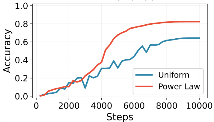
Arithmetic Task
